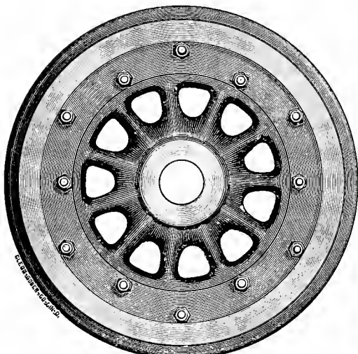
Figs. 5312-5213. Wheel for Engine-truck. Cast-iron Spoke-center. Tire secured by a Steel Retaining-ring. PAIGE CAR WHEEL COMPANY.
